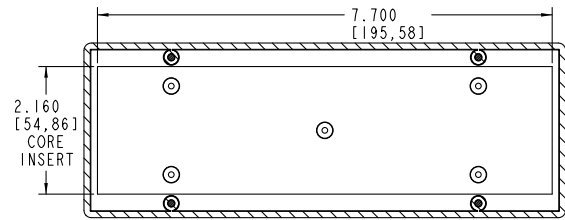
SECTION D-D INSERT FOR TOP & BOTTOM COVER
