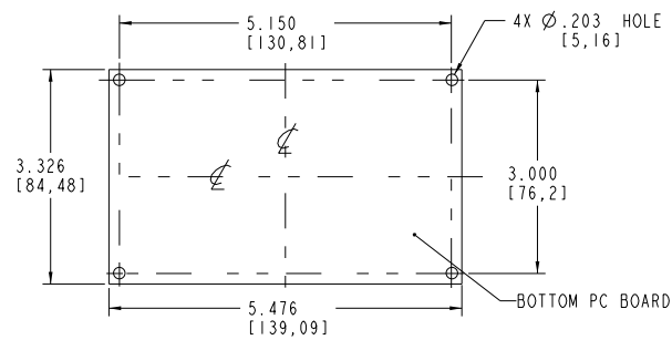
RECOMMENDED PC BOARD SIZE
