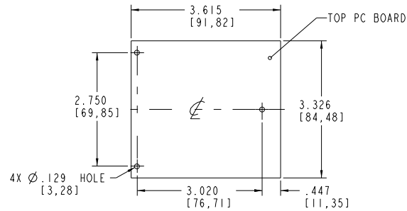
RECOMMENDED PC BOARD SIZE
