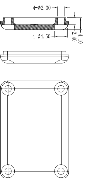
SECTION B-B
